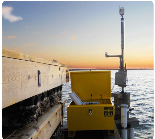
Portable aluminum chest monitoring system containing a YSI Bubbler, Sonde, Data Logger, and meteorological sensors.
