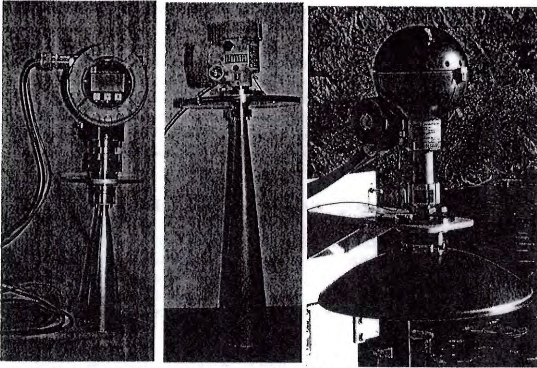
Figure 1. Pictured from left to right, Design Analysis Associates H-3611, Ohmart Vega Puls 62 and Saab Rosemount Tank Radar. Photos are not to scale.
