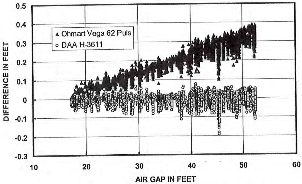
Figure 3. Difference between radar and float-well system plotted by air gap in feet.
