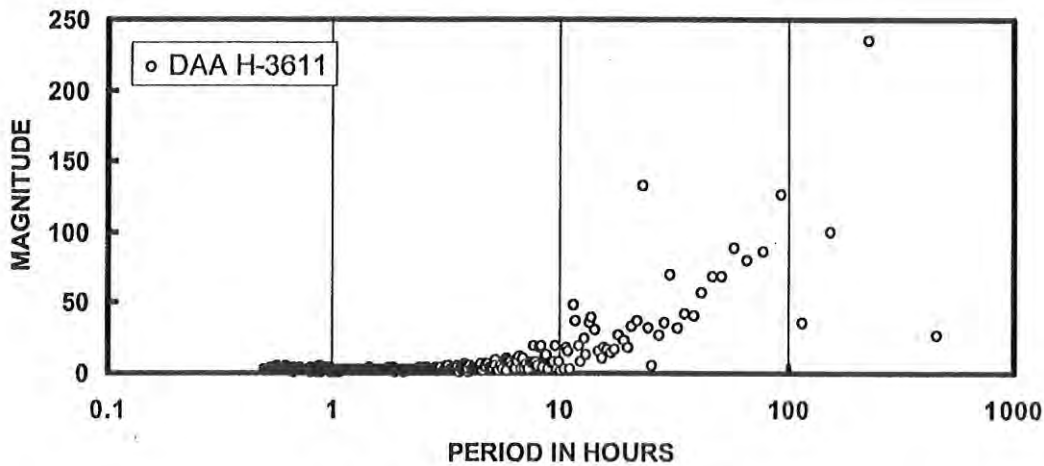
Figure 5. Plots of Fourier amplitudes of water-level data measured by a float-well system and a DAA H-3611 from September 15 at 15:45 to October 4 at 20:00 during drawdown of lake at Horse Mesa Dam.
